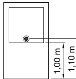
Figure 11.f - Door panel with glass panel above 1,0 m
