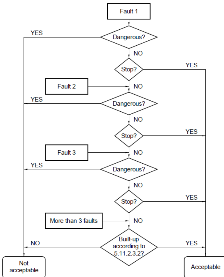
Figure 21 — Diagram for assessing safety circuits
