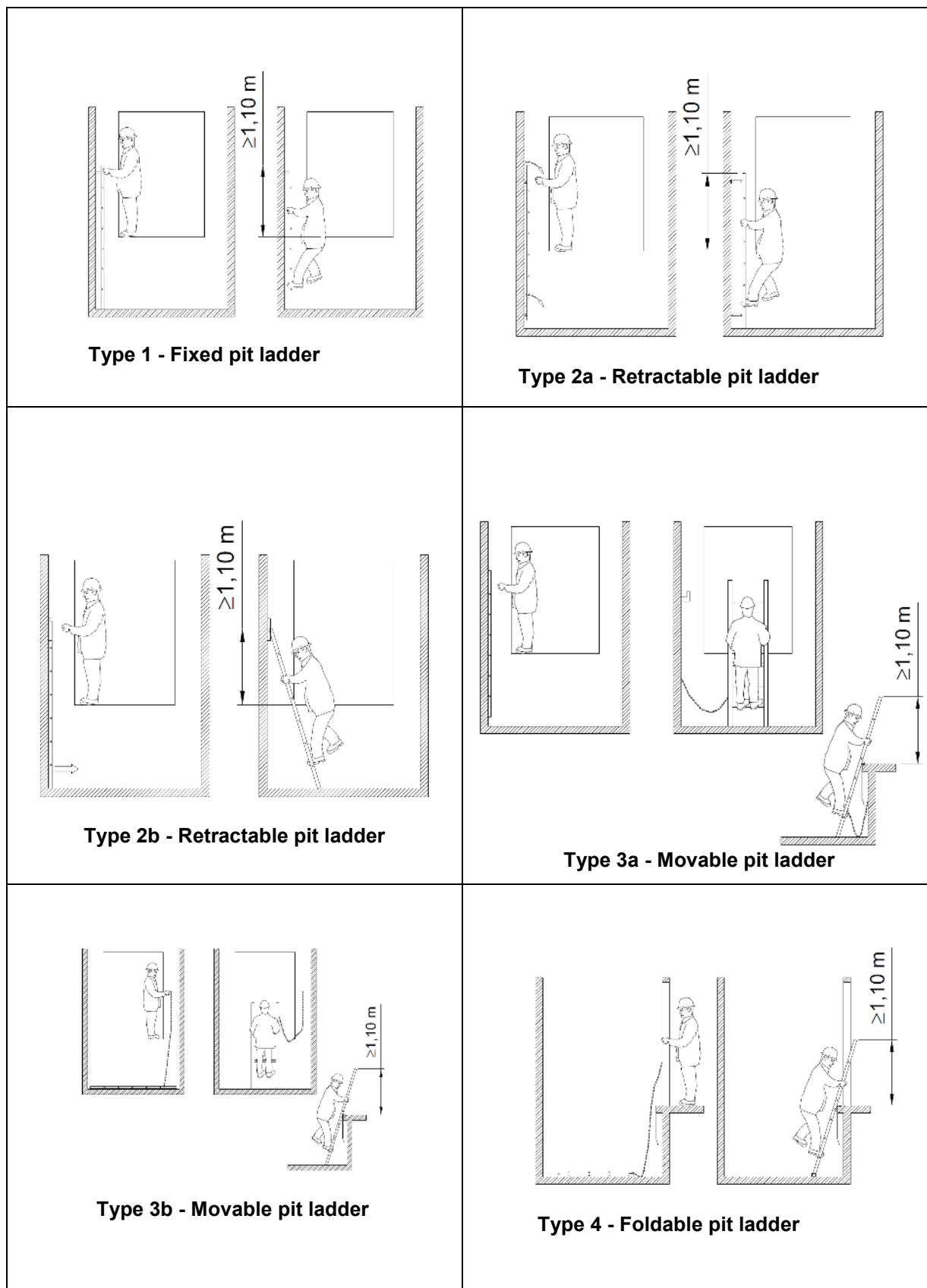
Figure F.1 — Types of pit access ladder
