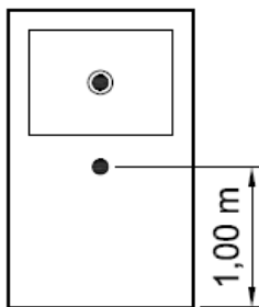
Figure 11.b - Door panel with glass panel
